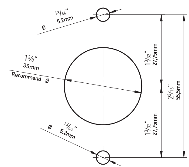
Fixing template
